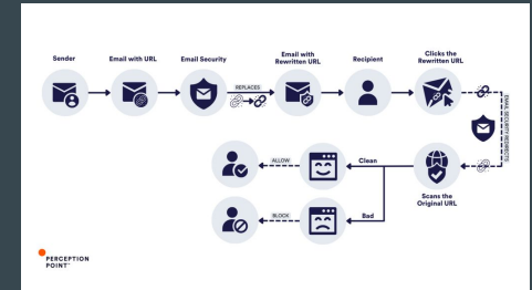
URL Link Scanning/Rewriting
